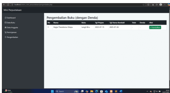
Gambar 7. Form Pengembalian
