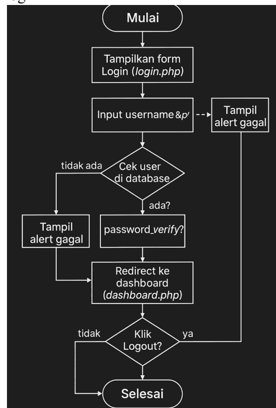
Gambar 1. Flowchart
